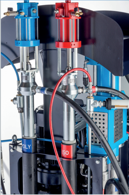
WIWA DUOMIX PU HYDRAULIC - with holders for the feed pumps
